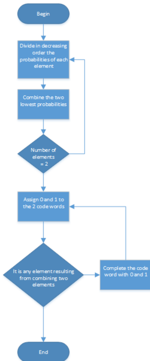
Fig. 1. Diagram of a Huffman Coding
